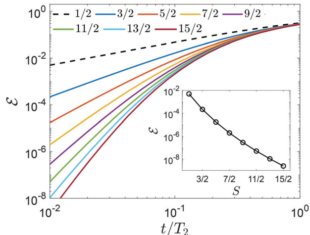
Fig. 1 Error \varepsilon after QEC as a function of the memory time t (in units of T_2 ), for different values of S . In this simulation, the system is prepared in the state |\psi_0\rangle = (|0_L\rangle + |1_L\rangle)/\sqrt{2} and evolves subject to pure dephasing for a time t . The capacity of the code increases with S , as shown in the inset for fixed t/T_2 = 10^{-2} .
