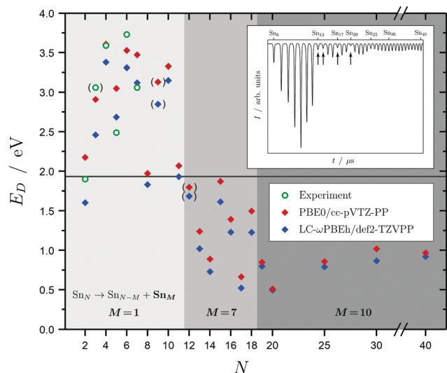
Fig. 2 Dissociation energies E_{\text{D}} in eV for the energetically most favorable fragmentation channels of the Sn N clusters with N = 2–20, 25, 30, 40 averaged over all isomers in the given energy range. Experimental values for the incremental dissociation energies are estimated based on atomization enthalpies obtained from Knudsen cell mass spectrometry. 14 The horizontal line at 1.9 eV gives the smallest accessible single-photon energy available in our photodissociation experiment. Over the size range studied, three regions can be distinguished: dissociation under the loss of an atom (light gray), a Sn 7 (gray) and a Sn 10 fragment (dark gray). Calculated dissociation energies in parentheses point to a differing fragmentation mechanism, i.e. , loss of a Sn 2 fragment for the Sn 9 parent cluster and loss of Sn 6 fragments for the Sn 12 parent cluster. The Sn 3 experimental dissociation energy in parenthesis has been evaluated assuming a linear geometry 12 (in its lowest 1 A 1 and 3 B 2 state Sn 3 is an isoscele triangle 21 ) and has thus to be considered with care. The inset shows a typical time-of-flight mass spectrum after F 2 excimer laser photoionization (7.89 eV) of the Sn N clusters given as arbitrary intensity I in dependence of the flight time t ; the naturally low-abundant clusters Sn 13 , Sn 14 , Sn 17 and Sn 20 are highlighted by arrows.
