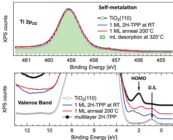
Fig. 11 Upper panel: Normalized photoemission spectra of the Ti 2p_{3/2} core level for a clean r\text{-TiO}_2(110) surface (open markers), after RT deposition of 1 ML of 2H-TTP (blue line) and after annealing to 200 °C (red line). For comparison, the spectrum measured on a monolayer obtained by desorption of a multilayer at 320 °C is also shown (green shaded area). Lower panel: Photoemission spectra of the valence band measured on the same substrate and films of the upper panel. The arrows mark the substrate DS peak and the 2H-TTP bulk HOMO state. Adapted from ref. 47 with permission from the American Chemical Society, Copyright 2017.
