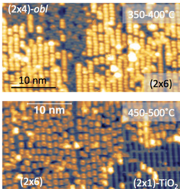
Fig. 16 Top: STM image (Colibri tip) showing the coexistence of (2 × 4)-obl and (2 × 6)-rect phases, as obtained by thermal desorption at 350–400 °C of a bi-layer film grown at RT (+2.5 V, 60 pA); molecules in the new phase display two symmetric lobes, much brighter than those in the (2 × 4)-obl phase. Bottom: The same film after annealing to 450–500 °C, as imaged close to a (2 × 1) reconstructed region, which shows a significant dewetting (+1.5 V, 80 pA).
