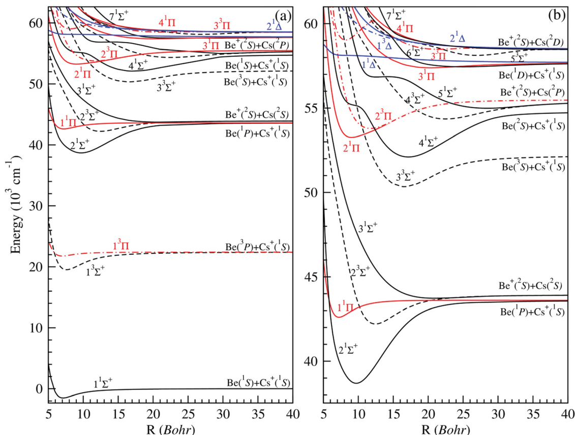
Fig. 1 Potential energy curves of singlet and triplet electronic states in Σ + , Π and Δ symmetries of the BeCs + molecular ion (panel (a)). Zoomed-in view of the higher excited states (panel (b)).
