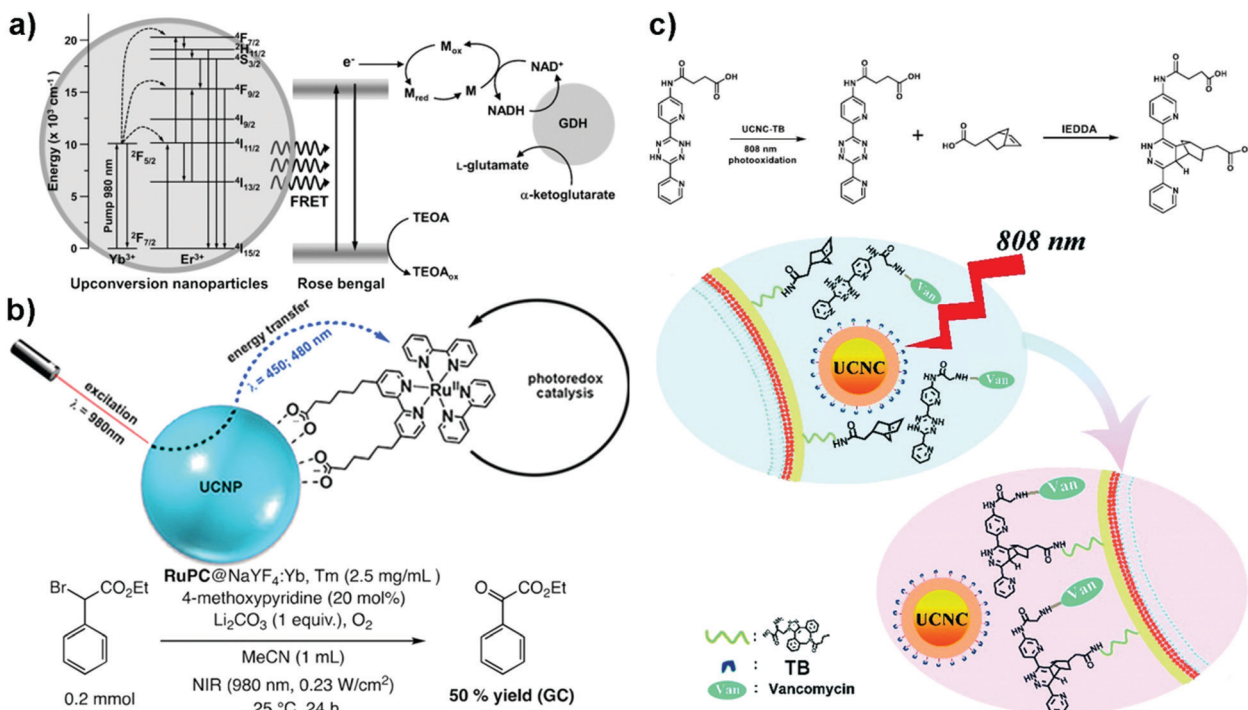
Fig. 3 (a) NIR-driven photoenzymatic catalysts combining \text{NaYF}_4:\text{Yb}^{3+},\text{Er}^{3+} , Rose Bengal (RB), a rhodium(III)-based mediator ( \text{M} ), nicotinamide adenine dinucleotide ( \text{NAD}^+ ) and L-glutamate dehydrogenase (GDH). 15 Reprinted with permission from ref. 15. Copyright 2014, Wiley-VCH. (b) NIR-driven photocatalyst combining \text{NaYF}_4:\text{Yb}^{3+},\text{Tm}^{3+} and a heteroleptic derivative of [\text{Ru}(\text{bpy})_3]^{2+} . 16 Reprinted with permission from ref. 16. Copyright 2018, Wiley-VCH. (c) NIR-driven photocatalyst combining \text{NaYF}_4:\text{Nd}^{3+},\text{Yb}^{3+},\text{Er}^{3+} and \text{NaYF}_4:\text{Nd}^{3+} and Toluidine Blue O (TB). 17 Reprinted with permission from ref. 17. Copyright 2021, Royal Society of Chemistry.
