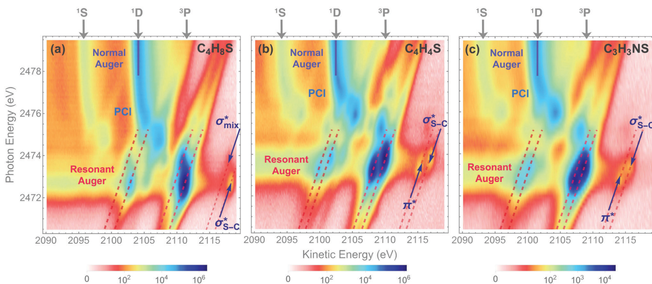
Fig. 3 2D maps of Auger S\ KL_{2,3}L_{2,3} spectra recorded in (a) thiolane, (b) thiophene, and (c) thiazole. The labels {}^1S , {}^1D , and {}^3P show the multiplet lines corresponding to the terms of the 2p^{-2} final-state configuration in the normal Auger spectra. Solid blue lines highlight the strongest 2p^{-2} ( {}^1D ) multiplet line. The areas of resonant KLL Auger spectra are indicated with dashed red lines around the photon energy of 2473 eV. The 2p^{-2}V({}^3P) final states corresponding to the first two excited states are labelled in the 2D maps.
