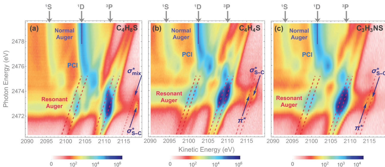
Fig. 3 2D maps of Auger S KL_{2,3}L_{2,3} spectra recorded in (a) thiolane, (b) thiophene, and (c) thiazole. The labels ^1S , ^1D , and ^3P show the multiplet lines corresponding to the terms of the 2p^{-2} final-state configuration in the normal Auger spectra. Solid blue lines highlight the strongest 2p^{-2} ( ^1D ) multiplet line. The areas of resonant KLL Auger spectra are indicated with dashed red lines around the photon energy of 2473 eV. The 2p^{-2}V(^3P) final states corresponding to the first two excited states are labelled in the 2D maps.
