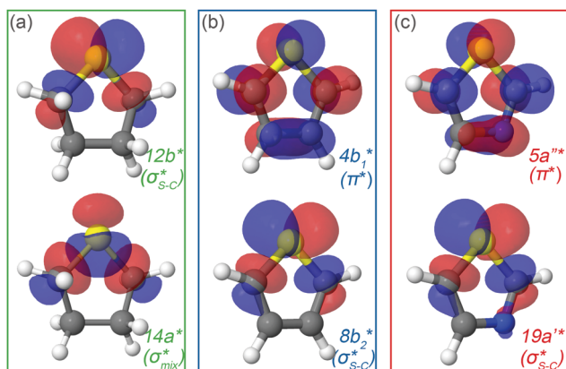
Fig. 2 Natural orbitals obtained at the IS-MCSCF level for (a) thiolane in twisted conformation, (b) thiophene and (c) thiazole corresponding to S 1s \rightarrow LUMO/LUMO+1 excitation.
