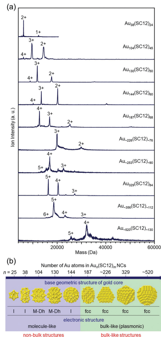
Fig. 5 (a) Positive-ion ESI mass spectra of Au n (SC12) m NCs. (b) Non-bulk to bulk transition between Au 144 (SC12) 60 and Au 187 (SC12) 68 in the Au n (SC12) m -NC system. 109 Reproduced with permission from ref. 109. Copyright 2015 American Chemical Society.
