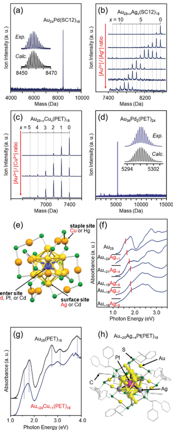
Fig. 6 Negative-ion MALDI mass spectra of (a) Au 24 Pd(SC12) 18 , 110 (b) Au 25-x Ag x (SC12) 18 , 111 and (c) Au 25-x Cu x (PET) 18 . 112 (d) Negative-ion ESI mass spectrum of Au 36 Pd 2 (PET) 24 . 114 (e) Preferential substitution site in Au 25 (SR) 18 for each element. 116 Blue, yellow, and orange spheres represent Au atoms, and green spheres represent S atoms. The R groups are omitted for clarity. Optical absorption spectra of (f) [Au 25-x Ag x (SC12) 18 ] - and (g) [Au 25-x Cu x (PET) 18 ] - . 112,158 (h) Geometric structure of [Au 20 Ag 4 Pt(PET) 18 ] 0 . 117 Reproduced with permission from ref. 110–112, 114, 116 and 117. Copyright 2010 The Royal Society of Chemistry, 2012 American Chemical Society, 2012 The Royal Society of Chemistry, 2016 The Royal Society of Chemistry, and 2018 American Chemical Society.
