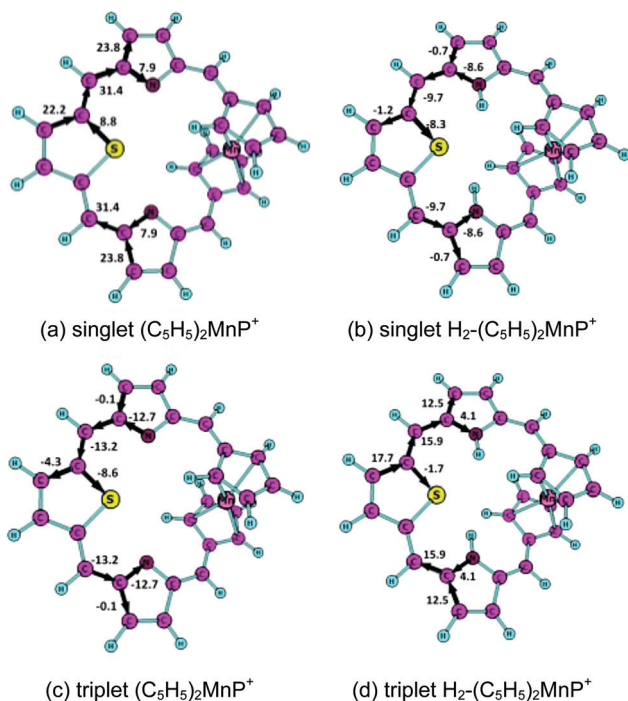
Fig. 7 The strength of the MIRC (in nA T -1 ) along selected bonds in (a) the singlet state of (C 5 H 5 ) 2 MnP + , (b) the singlet state of H 2 -(C 5 H 5 ) 2 MnP + , (c) the triplet state of (C 5 H 5 ) 2 MnP + and (d) the triplet state of H 2 -(C 5 H 5 ) 2 MnP + .
