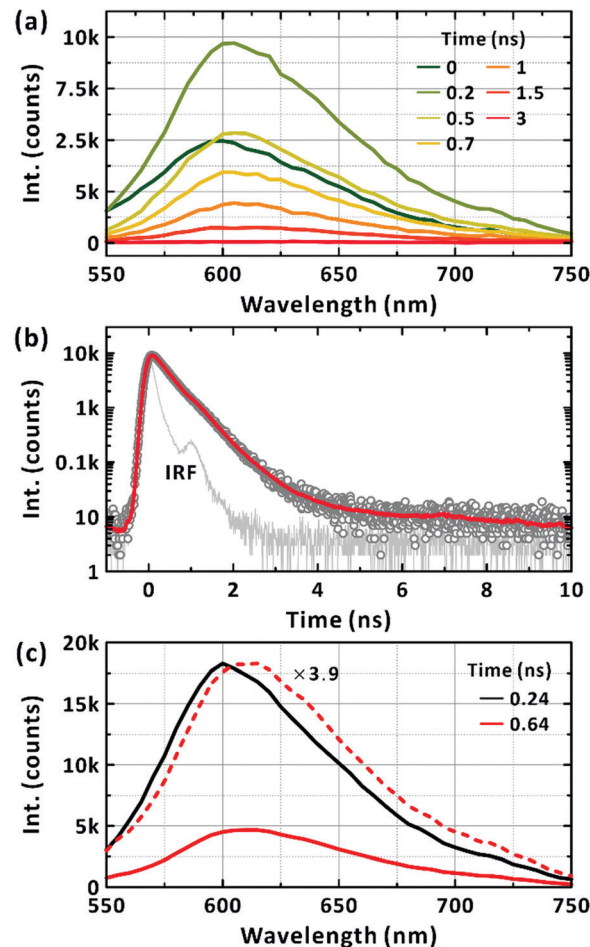
Fig. 3 Picosecond-resolved photoluminescence (PL) of PM6 in the \text{CHCl}_3 . (a) Time-resolved PL spectra of a minor conformation. Excitation wavelength is 510 nm. Representative time delays are given in the panel. (b) PL emission kinetic profiles monitored at 600 nm. The red solid line is the bi-exponential fit. Instrumental response function is also presented in the panel. (c) Lifetime-associated spectra. The two global-lifetime components of 0.24 ns (black) and 0.64 ns (red) are deconvoluted.
