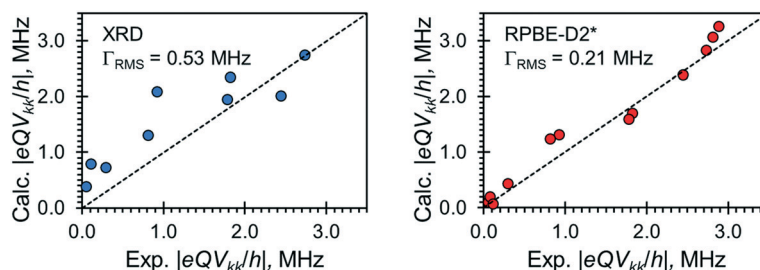
Fig. 3 Correlations between calculated and experimental principal components of ^{35}\text{Cl} EFG tensors for the four \text{NR}_4\text{Cl}:\text{xUrea}:\text{yH}_2\text{O} ( R = \text{Et, Pr} ; x = 1, 2, 3 ; y = 0, 1 ) MCCs. Computed EFG tensors are derived from calculations on the XRD-derived structures (blue) and structures with atomic coordinates refined at the RPBE-D2* level (red). \Gamma_{\text{RMS}} is the rms EFG distance, whereas the dotted lines represent perfect agreement between calculation and experiment.
