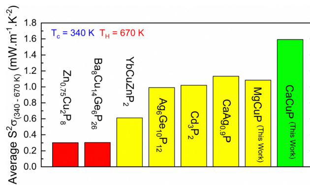
Fig. 4 Overview of temperature-average power factor \langle S^2/\rho \rangle for leading metal phosphide thermoelectrics. Data taken from: \text{Zn}_{0.75}\text{Cu}_2\text{P}_8 , 11 \text{Ba}_8\text{Cu}_{14}\text{Ge}_6\text{P}_{26} , 10 \text{YbCuZnP}_2 , 8 \text{Ag}_6\text{Ge}_{10}\text{P}_{12} , 6 \text{Cd}_3\text{P}_2 , 13 \text{CaAg}_{0.9}\text{P} . 14
