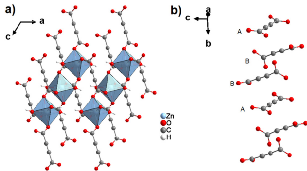
Fig. 46 Sections of the crystal structures of [Zn(ADC)(H 2 O) 2 ] (a) and [Ce 2 (ADC) 3 (H 2 O) 6 ] \cdot 2H 2 O (b), disclosing short C \equiv C \cdots C \equiv C contacts between neighbouring ADC ligands. The coordination sphere of Ce 3+ is omitted in (b) for clarity. Graphics redrawn from the cif file (CSD-Refcode DAYMAS and KAPHAL). 54,84
