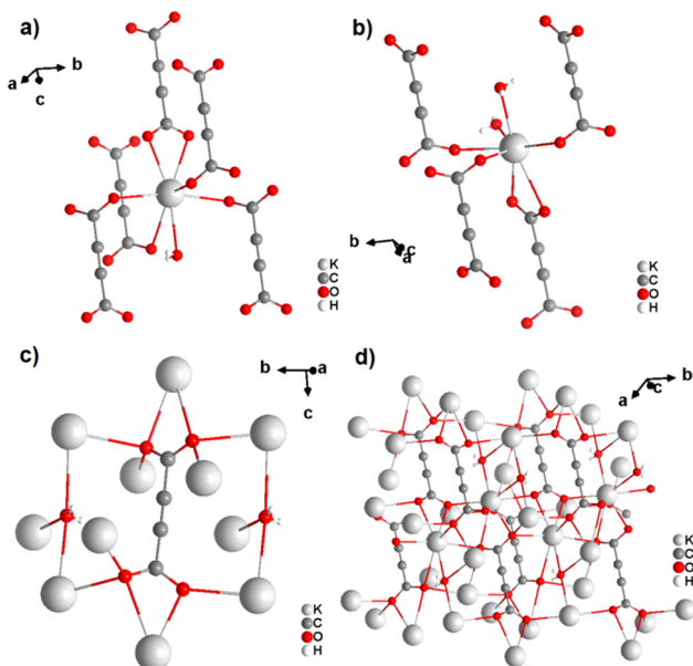
Fig. 6 Crystal structure of hydrated potassium acetylenedicarboxylate [K 2 (ADC)(H 2 O)] showing: (a) and (b) the coordination environment of the two crystallographically distinct K atoms, (c) the coordination mode of the ADC linker and water molecules, and (d) the complex three-dimensional framework structure. Graphics redrawn from the cif file (CSD-Refcode XADRUQ). 42
