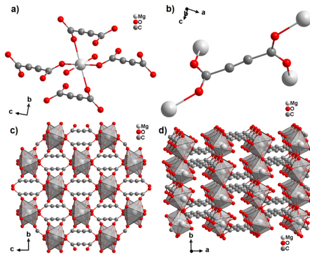
Fig. 7 Crystal structure of magnesium acetylenedicarboxylate [Mg(ADC)(H 2 O) 2 ] showing: (a) the coordination environment of the Mg atom, (b) the coordination mode of the ADC linker, and (c) and (d) the three-dimensional packing of the framework viewed along the [100] and [001] directions, respectively. Graphics redrawn from the cif file (Refcode GUWWOL). 45
