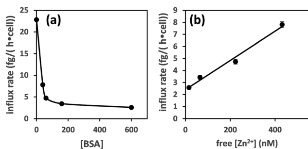
Fig. 3 Zinc influx depends on the concentration of albumin (a). This can be correlated to free [\text{Zn}^{2+}] for [\text{BSA}] = 40\text{--}600 \mu\text{M} (estimated using published stability constants for site A only; see ESI†) (b). The influx rate shows a linear relationship with free [\text{Zn}^{2+}] .
