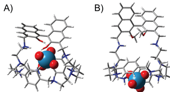
Fig. 4 Three-dimensional plots of the preferred conformers of (A) [1H_6(ReO_4)]^{5+} and (B) [2H_6(ReO_4)]^{5+} .
