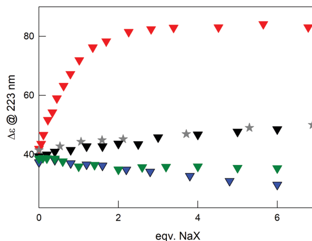
Fig. 3 Experimental titration profiles obtained from the CD titrations on [\text{1H}_6]^{6+} (0.1 mM) with solutions of different sodium salts (symbols: red, \text{NaReO}_4 ; blue, \text{NaNO}_3 ; green, \text{Na}_2\text{SO}_4 ; black triangles, \text{NaClO}_4 ; grey stars, \text{NaCl} ).
