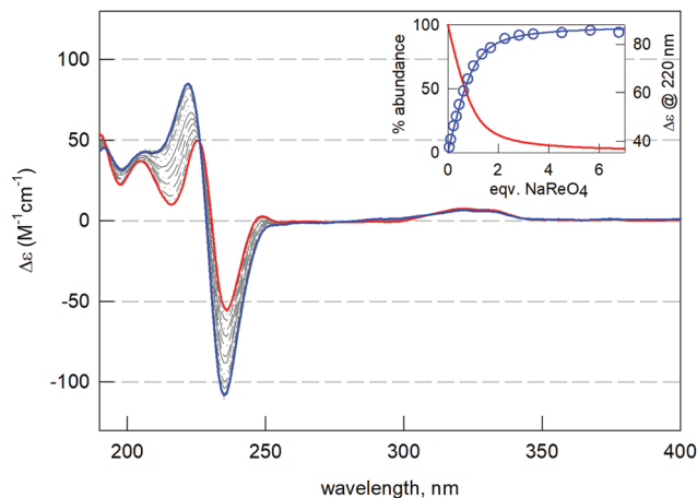
Fig. 2 CD titration of [\text{1H}_6]^{6+} (0.1 mM in 0.05 M \text{CF}_3\text{SO}_3\text{Na} , pH 2) with \text{NaReO}_4 (red and blue lines: initial and final spectra, respectively). Inset: Distribution diagram of the species (red line: % free [\text{1H}_6]^{6+} ; blue line: % [\text{1H}_6(\text{ReO}_4)]^{5+} ), superimposed to the experimental profile (circles).
