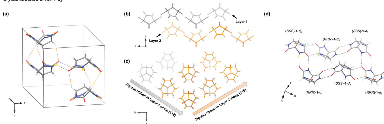
Crystal structure of (+)-(SSS)-1
