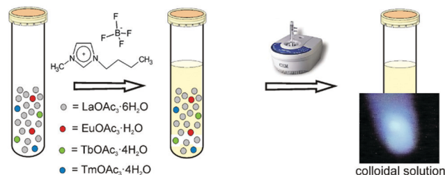
Fig. 12 Schematic illustration of the synthesis of light phosphors in ionic liquids in a microwave.
