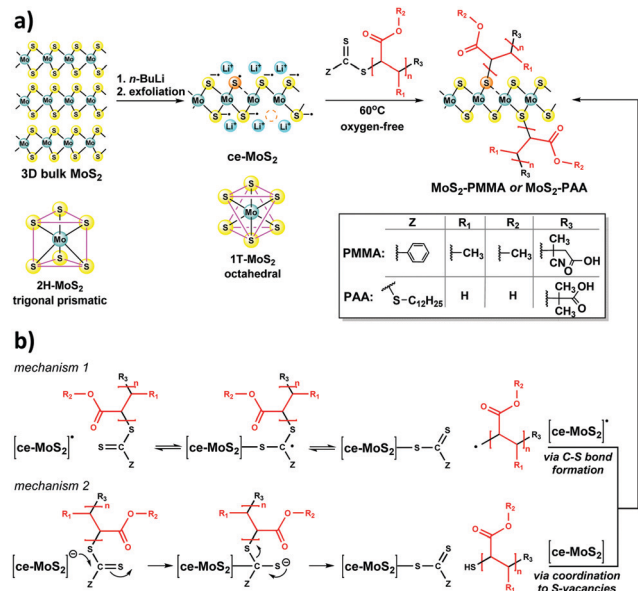
Fig. 1 Schematic illustration of the (a) chemical exfoliation of the bulk 2H-MoS 2 to 1T ce-MoS 2 and subsequent covalent functionalization with PMMA and PAA polymer chains. (b) Proposed reaction mechanisms furnishing MoS 2 -PMMA and MoS 2 -PAA ensembles.
