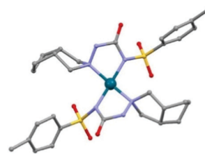
Fig. 1 Perspective view of [\text{Pd}(\text{glz})_2] . Hydrogen atoms are omitted for clarity.
