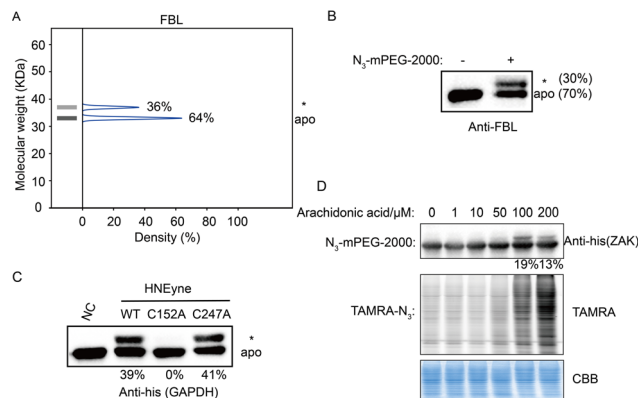
Fig. 4 Validation of the stoichiometry of HNE modification on individual proteins. (A) FBL is mono-modified by HNE with 36% stoichiometry in the STO-MS measurement. (B) The stoichiometry of FBL is determined to be 30% in an independent biochemical experiment. (C) C152 is the dominantly modified site in the case of GAPDH. In detail, compared to wildtype proteins, the mass shift totally disappears when C152 is mutated. However, no significant difference is observed when C247 is mutated. (D) Stoichiometry quantification of endogenous carbonylation on ZAK in arachidonic acid-treated cells.
