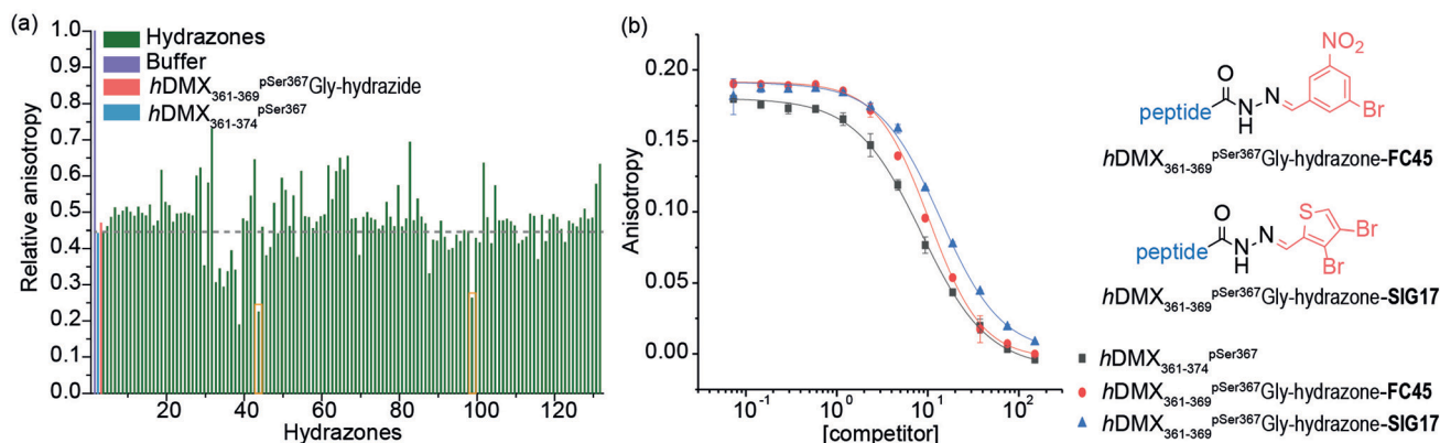
Fig. 2 Dynamic ligation screening based on hDMX 361-369 pSer 367 Gly-hydrazide (a) Anisotropy values of individually screened hydrazones (relative to buffer, zero activity negative control in grey), hDMX 361-374 pSer 367 (blue) and hDMX 361-369 pSer 367 Gly-hydrazide (red) as positive controls with hits (hDMX 361-369 pSer 367 Gly-hydrazide-FC45 and hDMX 361-369 pSer 367 Gly-hydrazide-SIG17) highlighted in orange boxes (10 \mu M acetylated hydrazide peptide mixed with 5 eq. of aldehyde, 1 \mu M 14-3-3 \eta , 50 nM hDMX 361-374 pSer 367 *, 50 mM NH 4 OAc, 10 mM aniline and 1 mM DTT) (b) competition FA curves for hydrazones taken forward as hits (50 nM hDMX 361-374 pSer 367 *, 1 \mu M 14-3-3 \eta in 50 mM NH 4 OAc, 10 mM aniline and 1 mM DTT).
