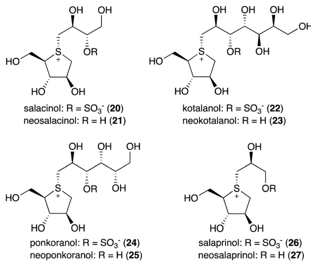
Fig. 4 Chemical structures of natural S -ribomimetics.
