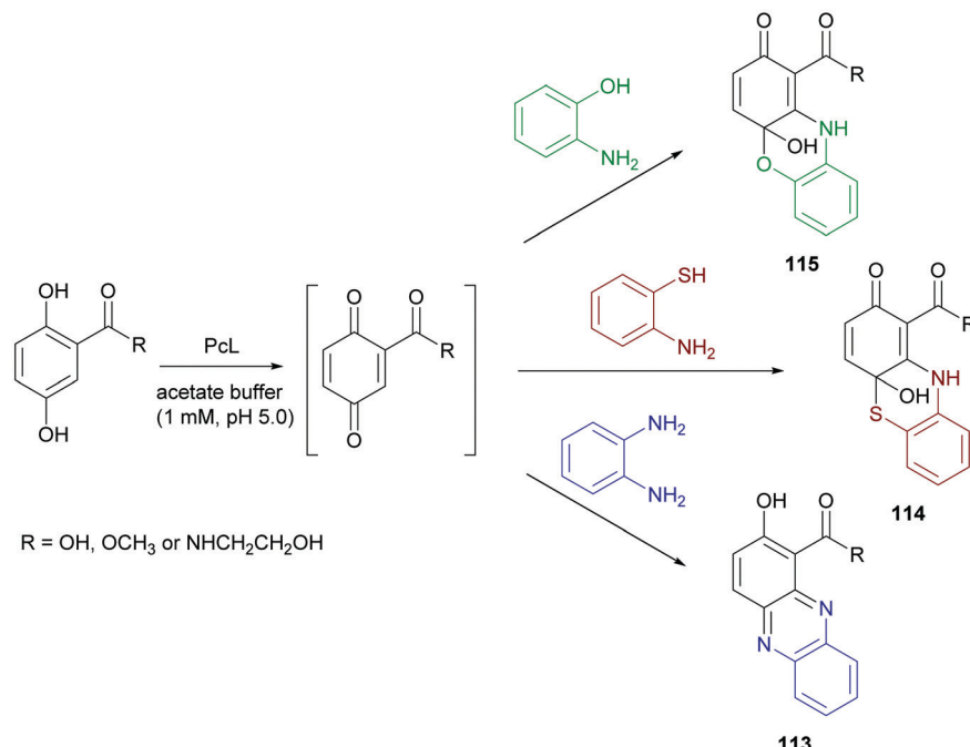
Scheme 21 Laccase-catalysed synthesis of phenazines, phenathiazines and phenoxazines.
