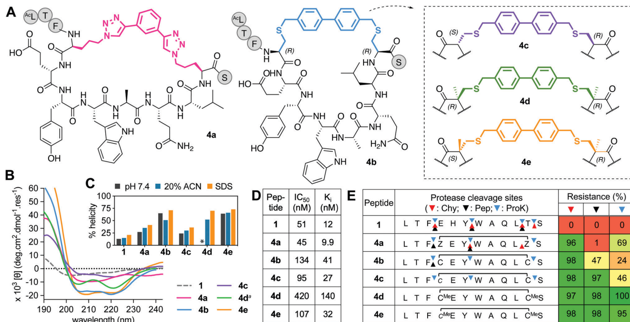
Fig. 4 A. Structures of aromatic ( i → i + 7)-crosslinked peptides 4a – 4e . B. CD spectra for 4a – 4e vs. 1 (50 μM) in 10 mM phosphate buffer (pH 7.4, 22 °C), except 4d in 20% ACN. C. Percent helicity calculated from CD spectra ( \theta_{220} ) in 10 mM phosphate buffer, 20% ACN or 20 mM SDS buffer (* not helical, Fig. S2, ESI†). D. IC 50 = mean peptide concentration to inhibit 50% binding of 1 -FITC (10 nM) to hDM2 (25 nM) measured by FP. pIC 50 ± SEM values are reported in Fig. S1, ESI†. Binding affinity (K i ) calculated from IC 50 values. E. Heatmap indicating percent peptide intact after 2 h incubation with chymotrypsin (Chy), pepsin (Pep) or proteinase K (ProK) at 22 °C and pH 8 or 2 (Pep only), measured by LCMS. Arrows show cleavage sites revealed by LCMS of the cleaved fragments.
