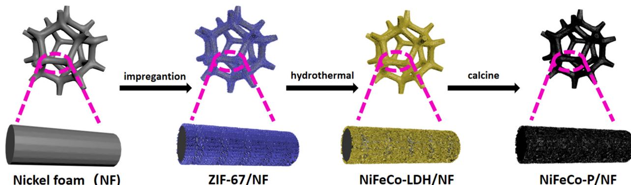
Scheme 1 Schematic illustration of the fabrication route of the NiFeCo-P/NF electrode.
