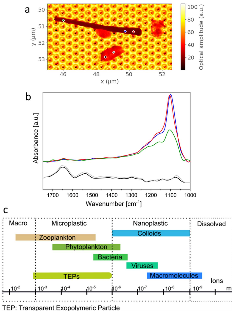
Fig. 5 (a) Optical scan and (b) nano-FTIR spectra of a typical, naturally occurring component in marine samples: \text{SiO}_2 -based fragments with strong bands around 1100\text{ cm}^{-1} and residues containing amide-groups with characteristic bands between 1700 and 1500\text{ cm}^{-1} , for example from proteins. (c) Size ranges of contents in natural marine samples.
