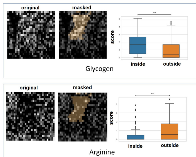
Fig. 6 Qualitative and quantitative comparisons between Raman chemical maps and CAIX map. For each chemical, the original chemical map, the chemical map masked with the hypoxia mask and the chemical score inside and outside the hypoxia region are presented from left to right.
