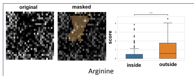
Fig. 6 Qualitative and quantitative comparisons between Raman chemical maps and CAIX map. For each chemical, the original chemical map, the chemical map masked with the hypoxia mask and the chemical score inside and outside the hypoxia region are presented from left to right.
