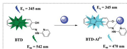
Scheme 1 Proposed mechanism for sensing Al 3+ .
