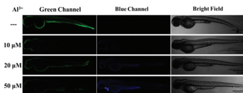
Fig. 5 Confocal fluorescence imaging of exogenous \text{Al}^{3+} in zebrafish. Top row: zebrafish were incubated with the probe BTD ( 5 \mu\text{M} ) for 60 min. Others: zebrafish were preincubated with 10, 20 and 50 \mu\text{M} \text{Al}^{3+} for 60 min and then incubated with the probe BTD ( 5 \mu\text{M} ) for 60 min, respectively. ( \lambda_{\text{ex}} = 405 \text{ nm} , \lambda_{\text{em}} = 440\text{--}500 \text{ nm} for the blue channel; \lambda_{\text{ex}} = 488 \text{ nm} , \lambda_{\text{em}} = 510\text{--}550 \text{ nm} for the green channel). Scale bar: 0.5 \text{ mm} .
