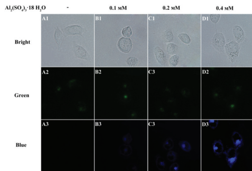
Fig. 4 Confocal fluorescence images of exogenous \text{Al}^{3+} in BEL-7402 cells. (A1–D3) The cells were incubated with the probe BTD ( 2.0 \mu\text{M} ) for 30 min and then incubated with 0.1 mM, 0.2 mM and 0.4 mM \text{Al}^{3+} for 30 min, respectively. ( \lambda_{\text{ex}} = 405 \text{ nm} , \lambda_{\text{em}} = 421\text{--}475 \text{ nm} for the blue channel; \lambda_{\text{ex}} = 458 \text{ nm} , \lambda_{\text{em}} = 500\text{--}550 \text{ nm} for the green channel.) Scale bar: 50 \mu\text{m} .
