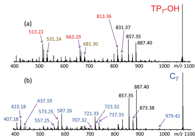
Fig. 5 LC-MS/MS spectra of the sodiated 7-mers ( m/z 1073.47) eluting at (a) 7.84 and (b) 8.57 min ( cf. Fig. 4 and Table S1 † ). Based on their elution order in RPLC, these eluates correspond to (a) TP_7 -OH and (b) C_7 , respectively.
