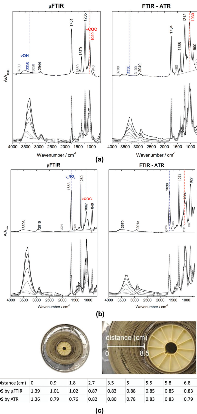
Fig. 9 Micro FITR ( \mu -FTIR) in transmission mode and ATR-FTIR spectra of (a) CA and (b) CN, where 3330, 1030 \text{cm}^{-1} and 1636, 1060 \text{cm}^{-1} are used to produce DS values. (c) DS values of CA of a historical reef from the inner parts to outer parts acquired using \mu -FTIR and ATR-FTIR. Reproduced with permission, 155 copyright (2020) Springer Nature.
