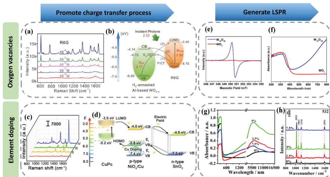
Fig. 9 (a) SERS spectra of R6G molecules adsorbed on WO_{3-x} substrate at different concentrations. (b) Schematic showing the energy level diagram of R6G on WO_{3-x} and the charge transfer process in this system. Reproduced with permission from ref. 103 (Copyright © 2019 WILEY-VCH Verlag GmbH & Co. KGaA, Weinheim). (c) SERS spectra of copper phthalocyanine (CuPc) molecules on Si(I), SnO_2 (II), SnO_2 -NiO (III), and Cu-doped SnO_2 -NiO (IV) substrates. (d) Schematic presenting the energy level diagram of CuPc on Cu-doped SnO_2 -NiO and the charge transfer process. Reproduced with permission from ref. 105 (Copyright © 2021 Wiley-VCH GmbH). (e) Electron paramagnetic resonance (EPR) spectra of the W_{18}O_{49} and WO_3 mesocrystals. (f) UV-vis spectra of W_{18}O_{49} and WO_3 mesocrystals. Reproduced with permission from ref. 25 (Copyright © 2021, American Chemical Society). (g) FTIR absorption spectra of Ga-doped ZnO nanoparticles combined with the UV-vis-NIR absorption spectra. (h) SERS spectra of MPy on Ga-doped ZnO substrate with different doping ratios. Reproduced with permission from ref. 107 (Copyright © 2021, American Chemical Society).
