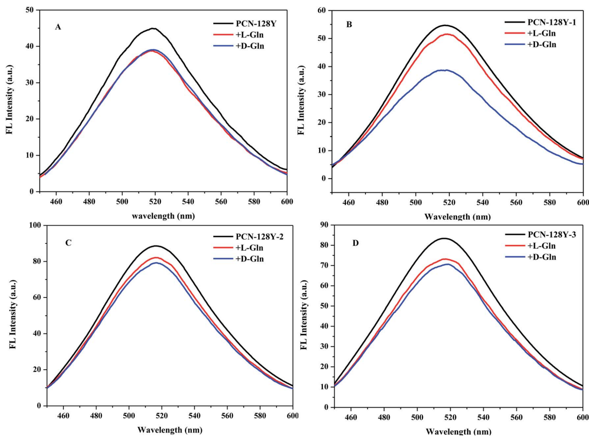
Fig. 9 Chiral fluorescence spectra of PCN-128Y (A), PCN-128Y-1 (B), PCN-128Y-2 (C), and PCN-128Y-3 (D) quenched by L/D-Gln (experimental conditions: 0.05 mg mL -1 MOFs, 50 \mu\text{L} 1 mol L -1 L- or D-Gln, 30 seconds incubation time, and 325 nm excitation wavelength).
