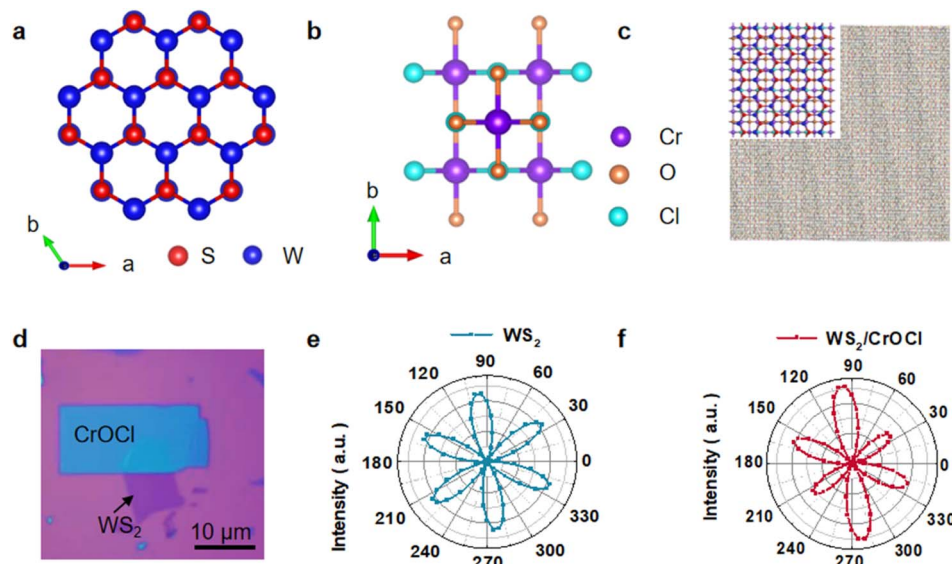
Fig. 1 Typical features of \text{WS}_2/\text{CrOCl} heterostructure. (a) Schematic illustrations of crystal lattice structure for \text{WS}_2 . (b) Schematic illustrations of crystal lattice structure for \text{CrOCl} . Red, blue, purple, orange and light blue spheres represent S, W, Cr, O and Cl atoms, respectively. (c) Moiré patterns of the \text{WS}_2/\text{CrOCl} heterointerface. The inset shows the corresponding lattice structure. (d) Optical microscope image of \text{WS}_2/\text{CrOCl} on \text{Si}/\text{SiO}_2 substrate. \text{WS}_2 flake on top of \text{CrOCl} flake. (e) Polar plot of angle-resolved second harmonic generation (SHG) pattern of \text{WS}_2 . (f) Polar plot of angle-resolved second harmonic generation (SHG) pattern of \text{WS}_2/\text{CrOCl} . Dots present the experiment data.
