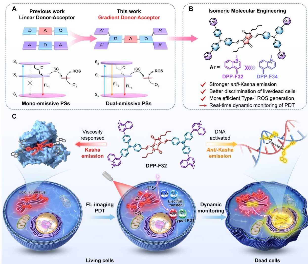
Scheme 1 (A) The gradient D-A structure facilitates the construction of dual-emissive PSs with anti-Kasha/Kasha behaviors. (B) Precise regulation through additional acceptor engineering. (C) Dual responses of DPP-F32 to DNA and viscosity for distinguishing live/dead cells and ratiometric monitoring of dynamic PDT.
