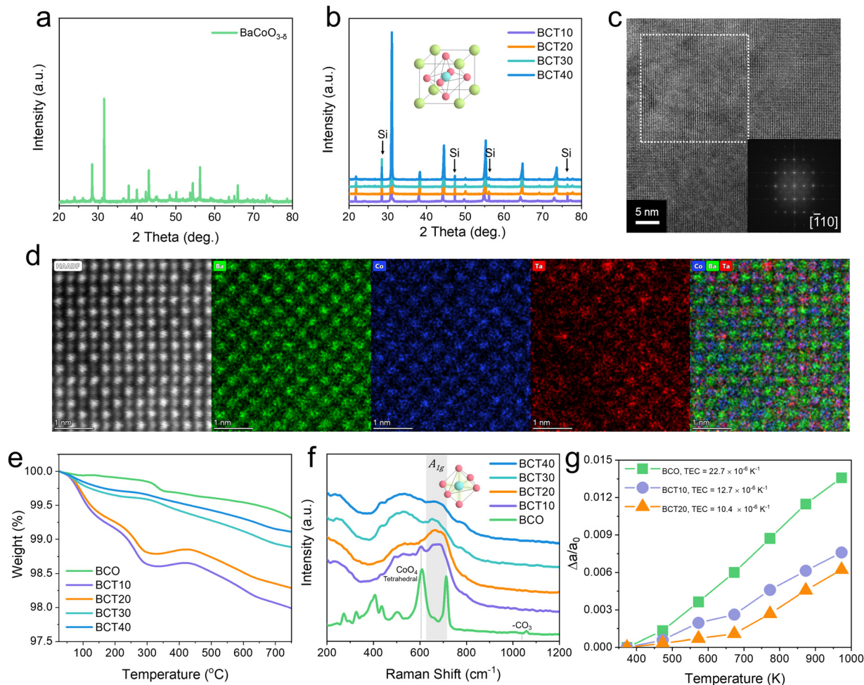
Fig. 1 X-ray diffraction (XRD) patterns of (a) as-synthesized barium cobaltites (BaCoO 3-δ , BCO) without B-site dopants and (b) Ta substituted barium cobaltites (BaCo 1-x Ta x O 3-δ , with X = 0.1, 0.2, 0.3, and 0.4). BCT10, BCT20, BCT30 and BCT40 denote the oxides having 10, 20, 30, and 40 mol% Ta in B-sites, respectively. It is noted that Si powder was deliberately added to serve as a reference peak (Si(111): 28.44°) for a more accurate analysis amongst the fabricated samples. (c) A high-resolution transmission electron microscopy (HRTEM) image of BCT20, (inset) fast Fourier transform (FFT) pattern. (d) Atomically resolved HAADF image of BCT20 and Elemental EDS maps for Ba, Co, Ta and overlaid. (e) Thermogravimetric profiles and (f) Raman spectra of BCT10, BCT20, BCT30 and BCT40. (g) The ratio of the thermally-expanded lattice parameters to the lattice parameters at 100 °C, Δa/a 0 , of BCO, BCT10, and BCT20 as a function of temperature.
