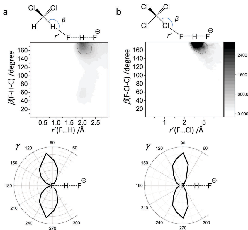
Fig. 8 The directionality of the intermolecular solvent-solute interactions: correlations between the intermolecular distance r' and the bond angle \beta . (a) \text{FHF}^- in \text{CH}_2\text{Cl}_2 ( \text{CH}\cdots\text{F} hydrogen bond). (b) \text{FHF}^- in \text{CCl}_4 ( \text{CCl}\cdots\text{F} halogen bond).
