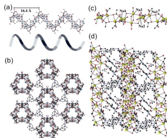
Fig. 1 (a) The 1D helical Li–O chain with a pitch of 16.4\text{ \AA} observed in IMP-24Li; (b) the projection view of the formed 1D Li–O chain along the [001] direction; (c) the structure presentation of 1D Na–O chain among IMP-27Na; (d) the projection view of the solvent-filled IMP-27Na along the [110] direction. Element color: C is black; O is red; Li is blue; Na is yellow. Reprinted with permission from ref. 42. Copyright 2018, American Chemical Society.
