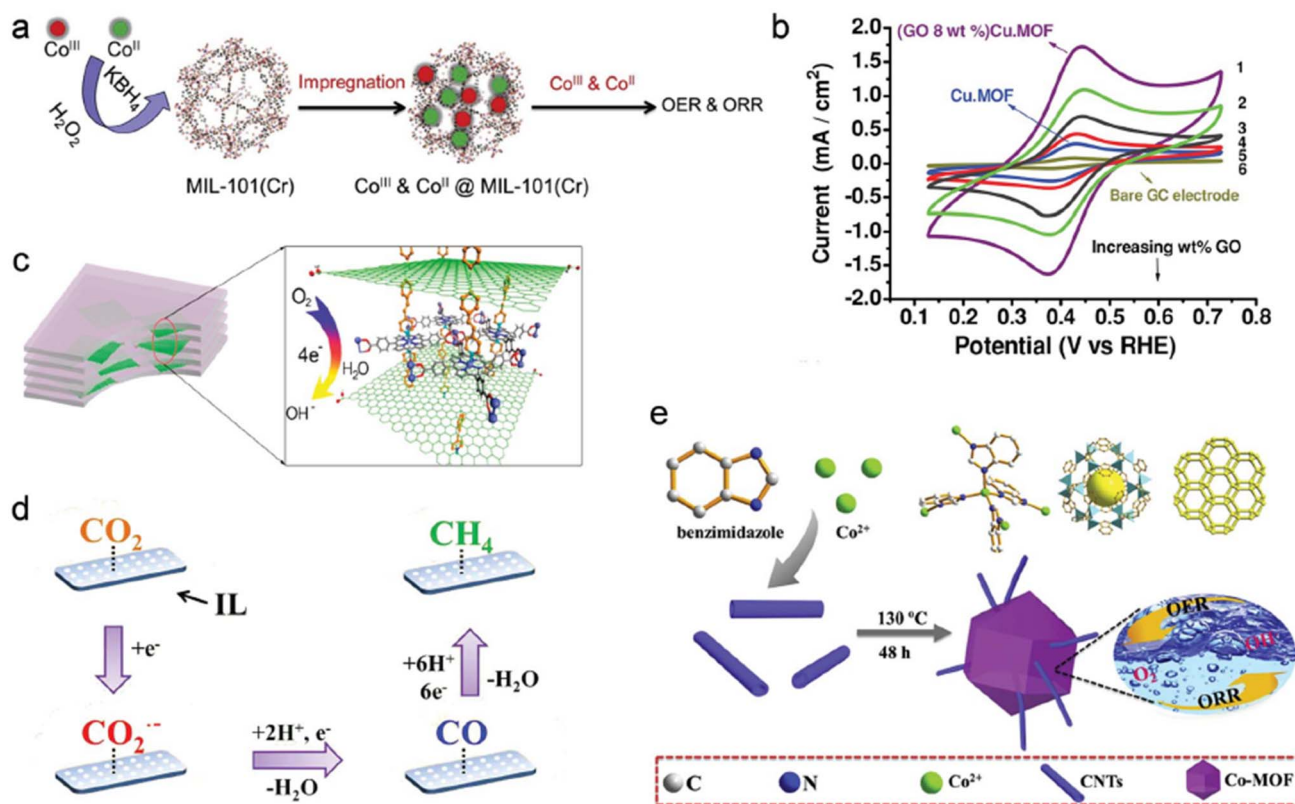
Fig. 7 (a) An example of the bifunctional electrocatalyst's design and preparation. (b) The catalysts' electrochemical activity, sorption surface areas, and surface areas. (c) A enlarged view of the layers inside the (\text{G-dye-FeP})_n MOF's framework and graphene sheets (d) an electrochemical procedure on the Zn-MOF/CP cathode in ionic liquids that might convert \text{CO}_2 to \text{CH}_4 (e) Co-MOF@CNTs catalyst synthesis. Copyrights 2019 from ref. 106.
