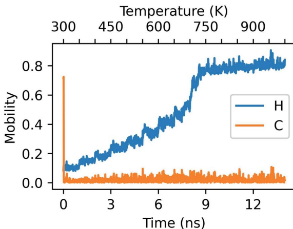
Fig. 6 Mobility descriptors for a randomly alloyed Au 1149 Pt 266 NA in the configuration of an lh which has been rapidly heated from 300 K to 1000 K over the span of 14 ns. \Delta t has been set to 10 ps.
