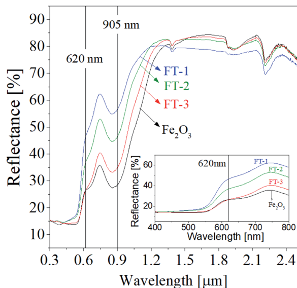
Fig. 9 UV-vis-NIR diffused reflectance of nanostructured \text{Fe}_2\text{O}_3/\text{TiO}_2 (FT-X) pigments calcined at 700^\circ\text{C} .
