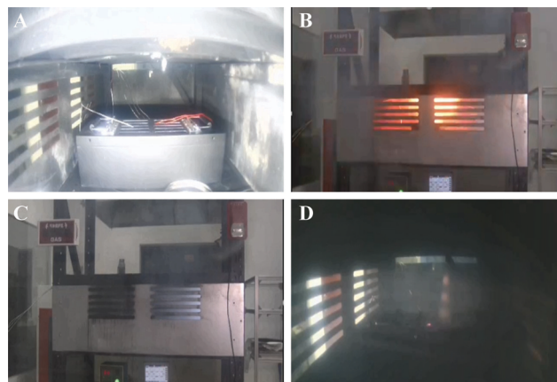
Fig. 6 Test chart of fire extinguishing capacity of (A) 32 650 \text{LiFePO}_4 batteries module (including module shell) in fire extinguishing experiment. (B) Thermal runaway fire of lithium-ion batteries module. (C) Extinguishing an open fire after spraying the extinguishing agent. (D) There is no reburning of the thermal runaway lithium-ion battery module.
