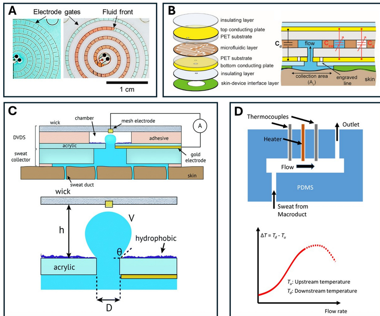
Fig. 5 Schematic overview of the presented flow rate measurement techniques (excluding the indirect derivation from the sweat composition). A ) Illustration of impedimetric measurement showing interdigitated electrodes in a spiral channel with a propagating fluid, reprinted with permission. 20 Copyright 2022, ACS Sens. B ) Illustration of a continuous capacitive flow rate sensor, where the microfluidic channel resides in between the conducting plates, changing the capacitance as result of different ratios of sweat ( C_{sw} ) and air ( C_a ). Reprinted with permission. 79 Copyright 2020, ACS Sens. C ) A schematic overview of a volume dispensing system, illustrating the droplet before an absorption event with the wick takes place. The height ( h ), contact angle ( \theta ) and diameter ( D ) of the opening influence the absorption frequency with a given flow rate. Reprinted with permission. 83 Copyright 2018, Lab Chip. D ) Illustration of the calorimetric method, consisting of a heater equally spaced between two thermocouples. Reprinted with permission. 90 Copyright 2018, Sensors.
