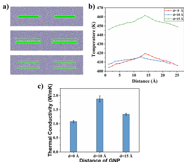
Fig. 13 (a) Molecular structure model of graphene/PEEK composites with different spacing of bilayer graphene ( d = 0 Å, d = 10 Å, d = 15 Å); (b) simulated temperature gradient of TC of graphene/PEEK composites with different spacings of bilayer graphene; (c) comparison of TC simulation results of graphene/PEEK composites with different spacings of bilayer graphene.
