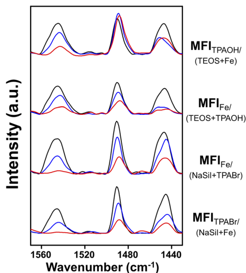
Fig. 2 FT-IR spectra of pyridine-adsorbed Fe-MFI samples. Spectra were measured after the desorption of pyridine at 150^\circ\text{C} (black line), 300^\circ\text{C} (blue line) and 500^\circ\text{C} (red line) for 1 h.
