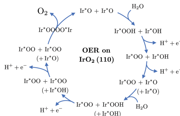
Fig. 2 Schematic of the catalytic cycle of the OER on \text{IrO}_2(110) according to the novel mechanism. For the dissociative adsorption of the second water molecule, a third surface oxygen entity is involved, indicated in brackets for the respective steps only.
