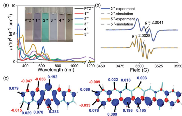
Fig. 3 (a) UV-vis-NIR absorption spectra of the radical cation species of PTZ •+ and 1 •+ –5 •+ . Inset: Photos of the solutions. (b) EPR spectra of 2 •+ and 5 •+ , and their simulations. (c) Calculated spin density distributions of 2 •+ (left) and 5 •+ (right).
