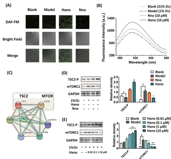
Fig. 4 (A) NO levels of blank, model and 10 μM Hano/Nno treated groups in situ detected with NO fluorescent probe DAF-FM DA (Ex: 495 nm, Em: 515 nm); (B) NO levels of Hano or Nno (10 μM) treated H9c2 cells under hypoxia (DAF-FM, Ex: 495 nm, Em: 515 nm); (C) protein–protein interactions between TSC2 and mTORC1 from the STRING database; (D) TSC2-P and mTORC1 protein expressions in H9c2 cells treated with or without 10 μM Hano or Nno; (E) TSC2-P and mTORC1 protein expressions in H9c2 cells treated with Hano (0–10 μM).
