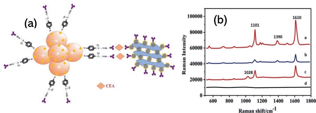
Fig. 8 (a) Schematic illustration of sandwich sensing assembly for CEA detection with SERS magnetic supporting substrate. (b) SERS spectra of MoS 2 -NFs@AuNPs/MBA (spectrum-a), MoS 2 -NFs@AuNPs/MBA/anti-CEA (CEA SERS tag) (spectrum-b), sandwich type immunosensor including 1.0 ng mL -1 CEA (spectrum-c) and anti-CEA/Fe 3 O 4 NPs@AuNPs/d-Ti 3 C 2 T x MXene (spectrum-d). Reproduced from ref. 144 after permission, copyright© 2020 Elsevier.
