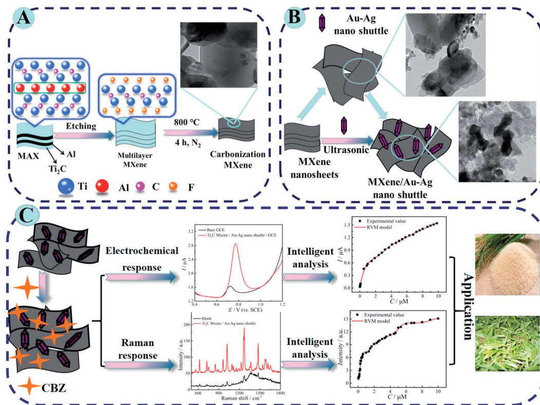
Fig. 9 (A) Synthesis of \text{Ti}_2\text{C} MXene and subsequent carbonization by annealing at 800\text{ }^\circ\text{C} under nitrogen protection. (B) Schematic fabrication of \text{Ti}_2\text{C} MXene/Au–Ag NSs. (C) Experimental and theoretical studies of bifunctional biosensing platform for electrochemical and Raman analysis for CBZ determination in tea and rice residues. Reproduced from ref. 174 after permission, copyright© 2020 Elsevier.
