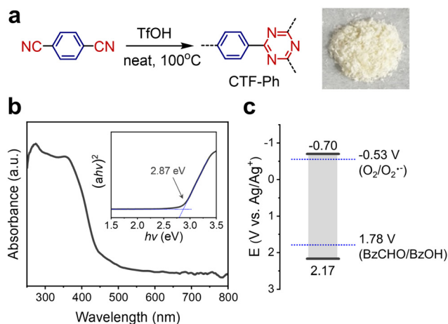
Fig. 1 (a) Solid-phase polymerization of CTF-Ph as an off-white powder. (b) UV-vis diffusion reflectance spectrum of CTF-Ph with an inset of the corresponding Tauc plot. (c) Electronic band structure of CTF-Ph determined by cyclic voltammetry.
