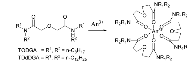
Scheme 10 DGA ligands for extraction in a SANEX flowsheets.
